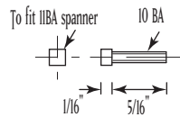
Coupling Rod Support Bolt (made from standard 10BA bolts) (4)
