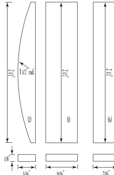
Deck Planks Matl. Ramin
