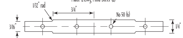
Buffer Strap Matl. 24swg Mild Steel (2)
